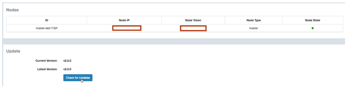
FIGURE 27 Updating software
